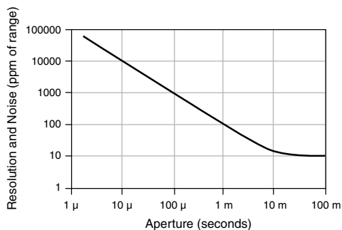
Figure 2. Noise and Resolution versus Measurement Aperture, Typical
