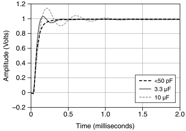
Figure 3. 10 mA Range Step Response, Typical
