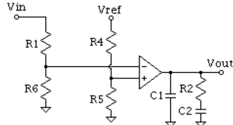
Transconductance
