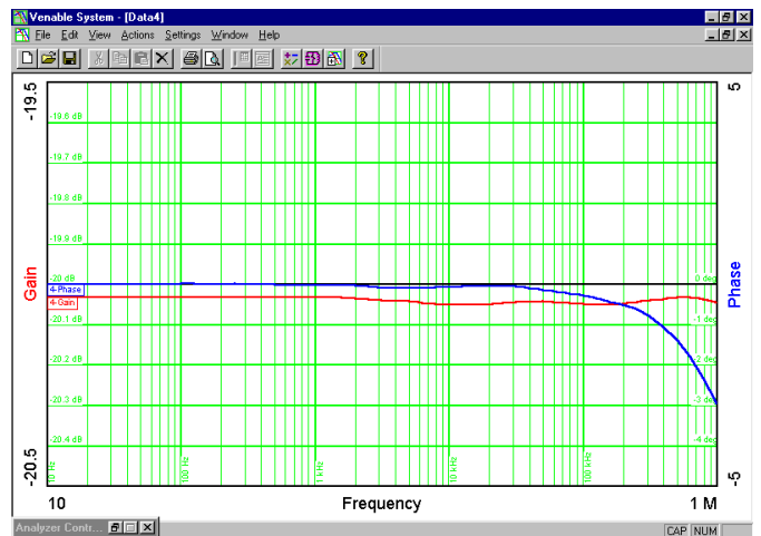
Transfer function of calibrated probe. The gain and phase deviations at 1 kHz are minimized. Note the narrow gain and phase ranges of the graph.
